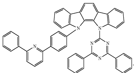
Compound E68
