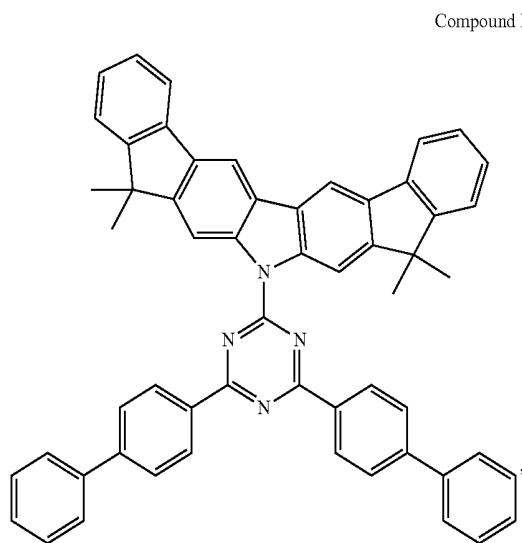
Compound E76
