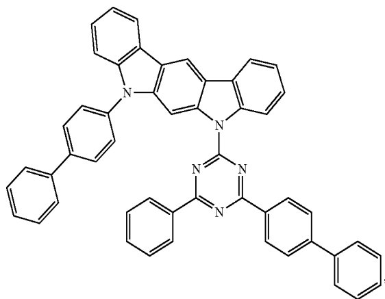
Compound E28
