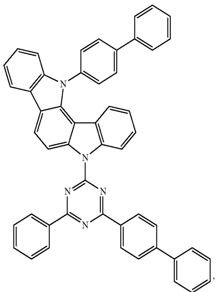
Compound E44
