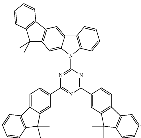
Compound E40
