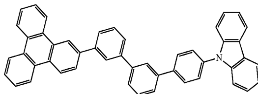
Compound 6
