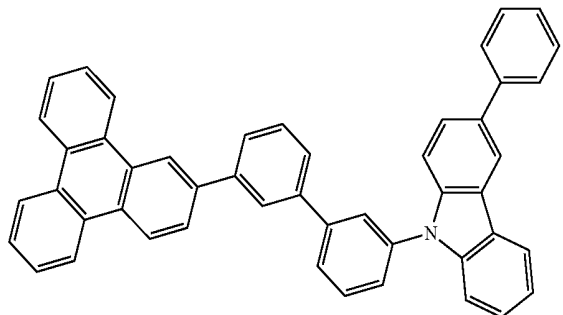
Compound 11
