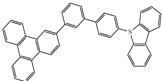
Compound 4
