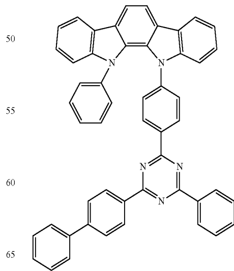
Compound E51
