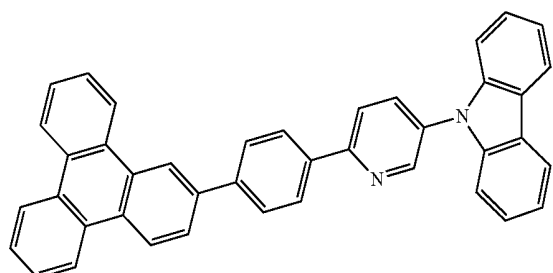
Compound 46
