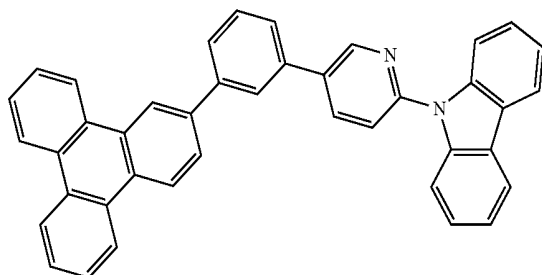
Compound 20
