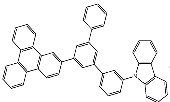
Compound 14
