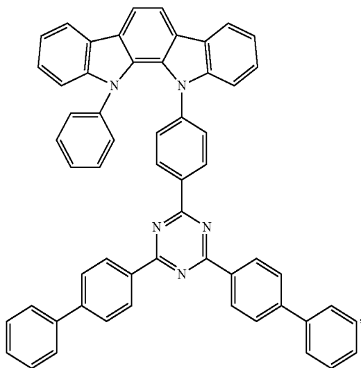
Compound E55
