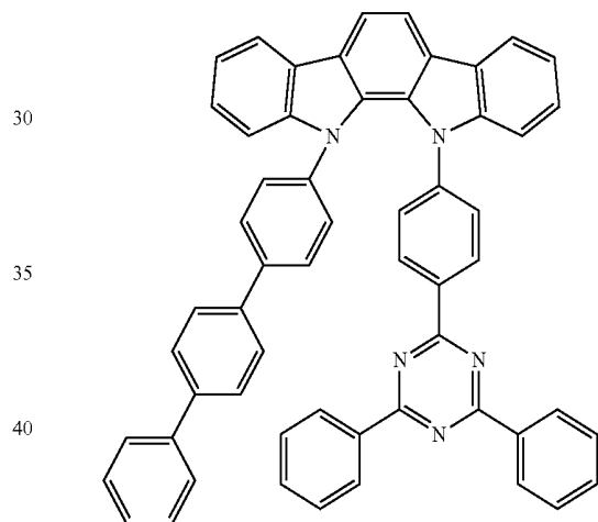
Compound E53
