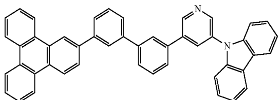
Compound 48
