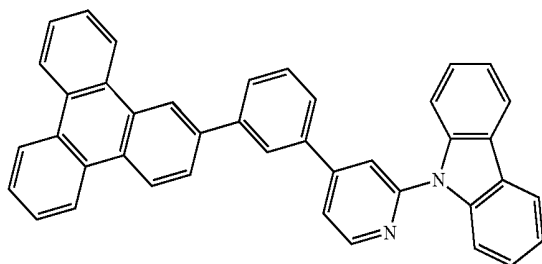
Compound 19
