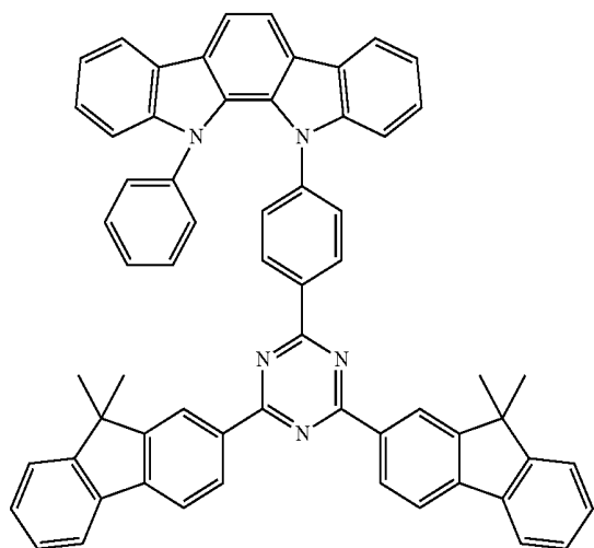
Compound E56
