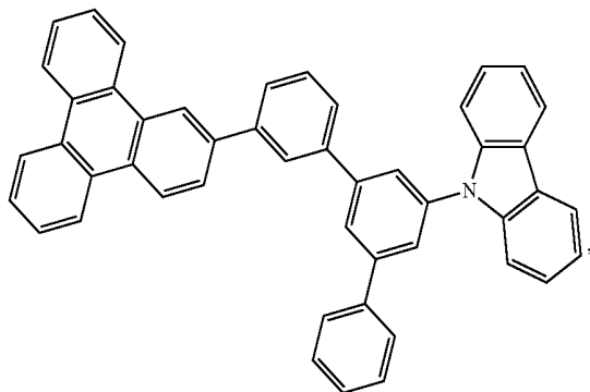
Compound 12
