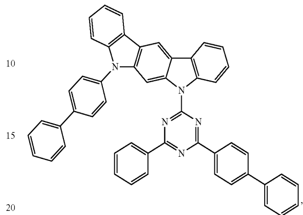
Compound E28
