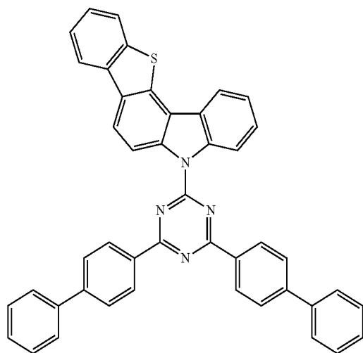
Compound E47
