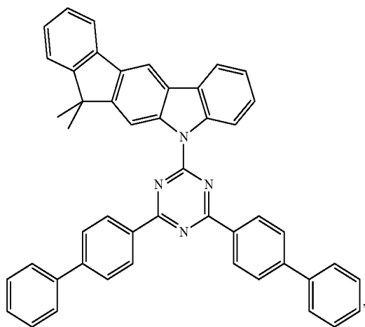
Compound E39
