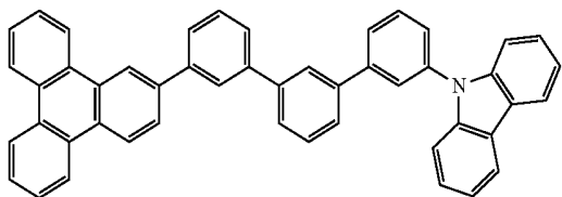
Compound 5
