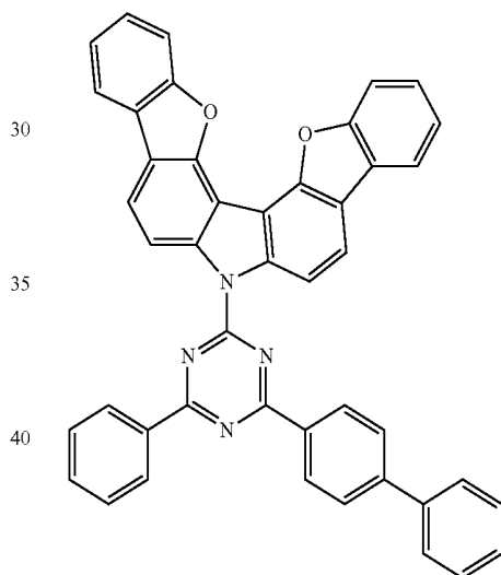
Compound E76
