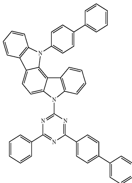
Compound E44
