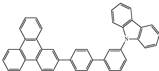
Compound 4
