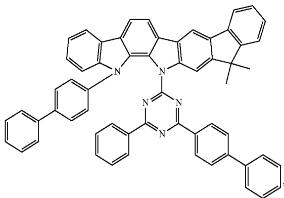
Compound E73
