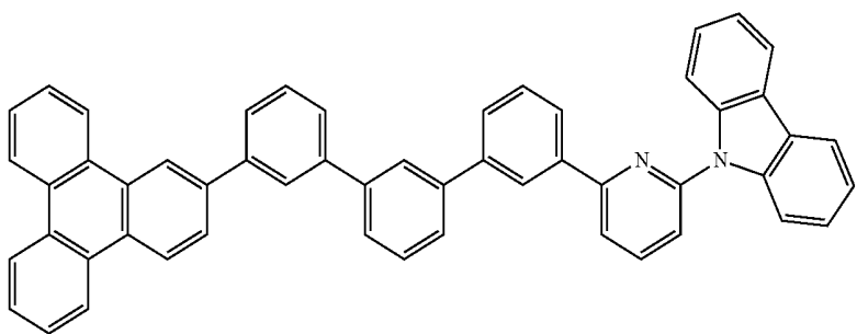
Compound 28
