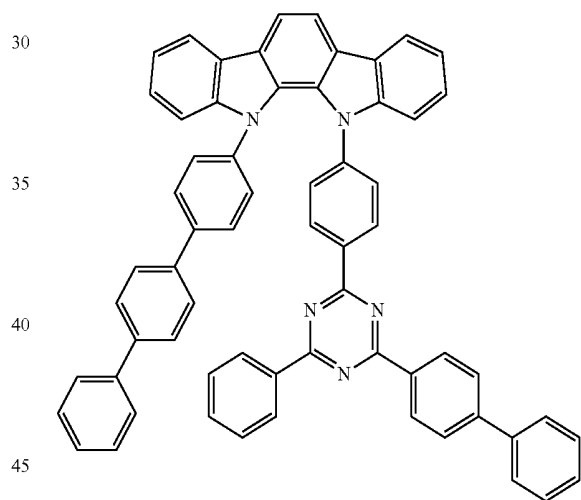
Compound E59
