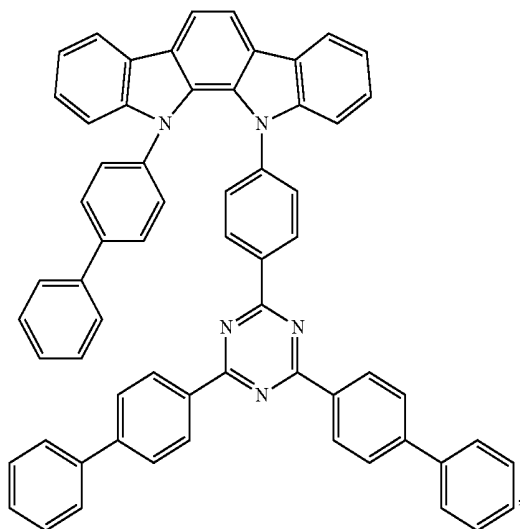
Compound E58
