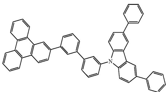
Compound 14
