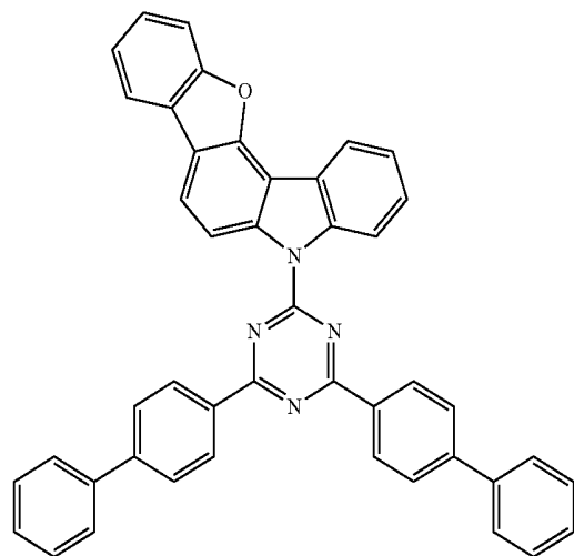
Compound E50
