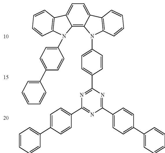
Compound E58
