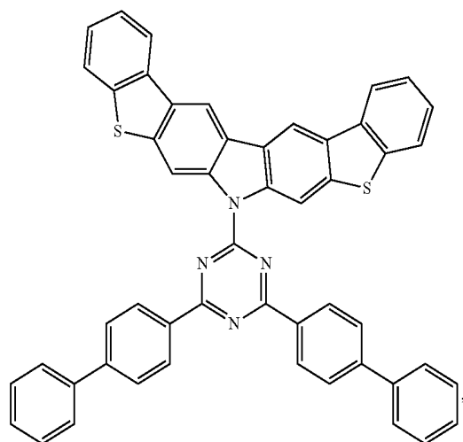
Compound E77
