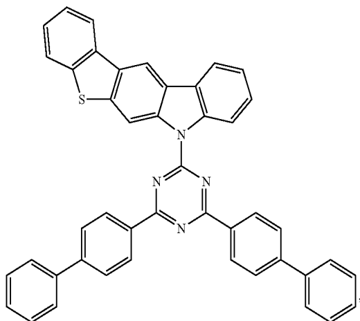
Compound E33
