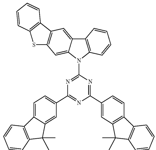
Compound E34
