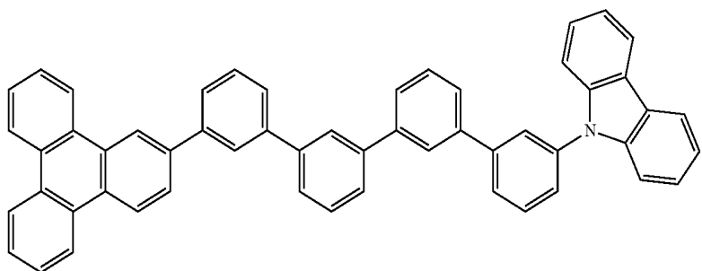
Compound 10
