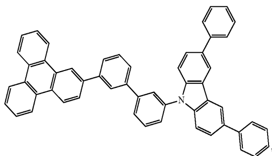
Compound 12
