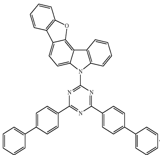
Compound E50
