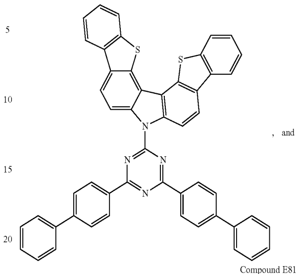
Compound E80
