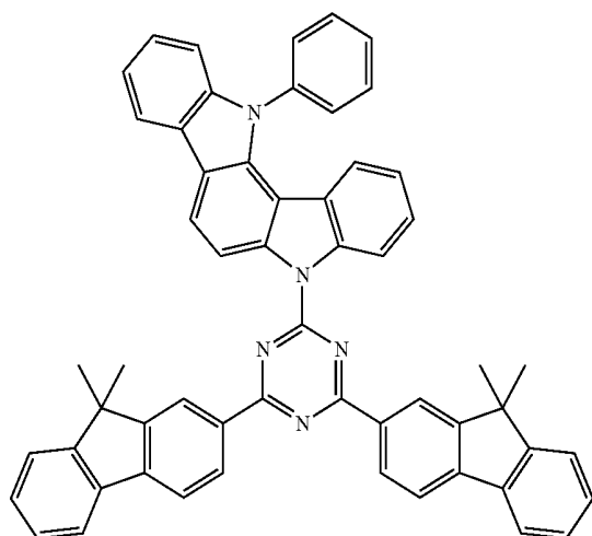
Compound E44
