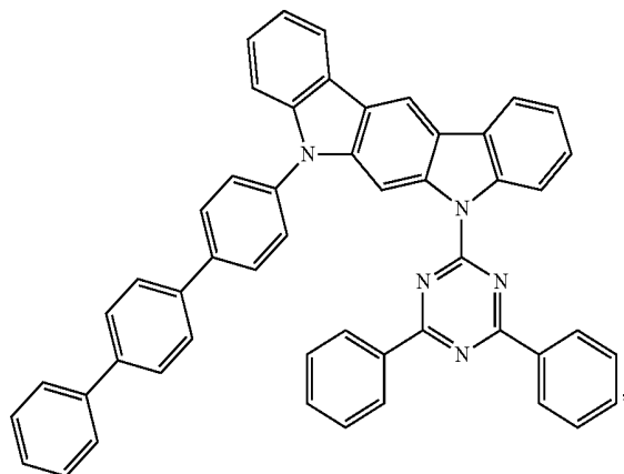
Compound E27 5
