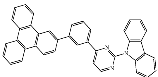
Compound 41
