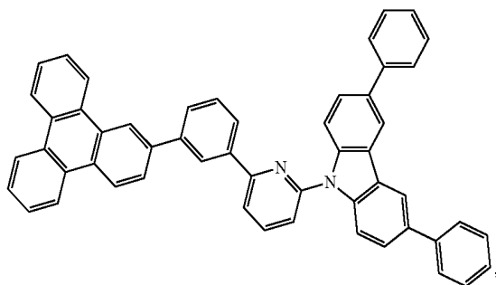
Compound 32
