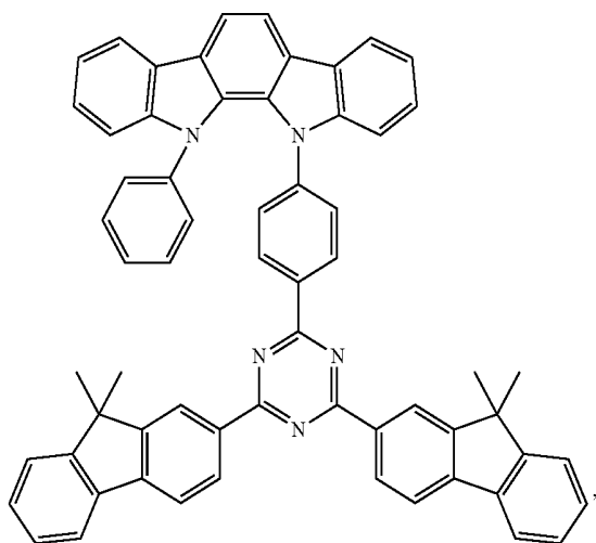
Compound E56
