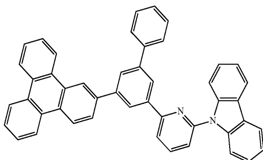
Compound 32
