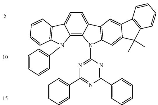
Compound E72
