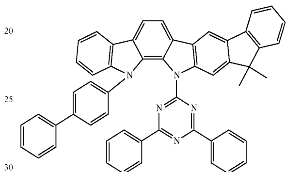
Compound E73
