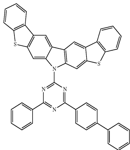
Compound E76
