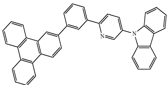
Compound 45
