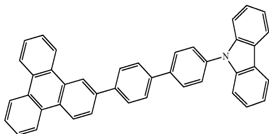
Compound 3
