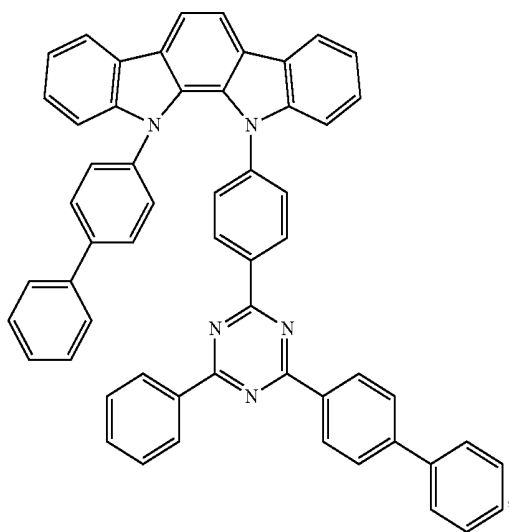
Compound E57
