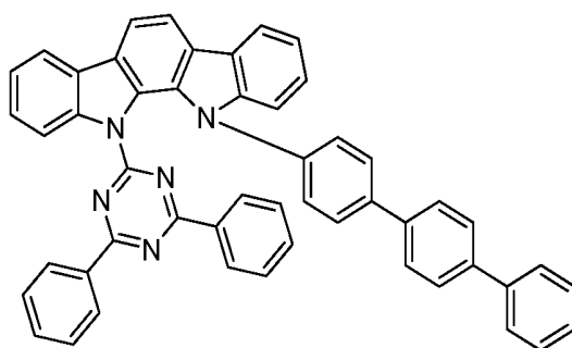
Compound E2
