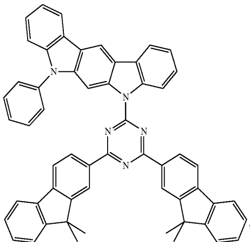
Compound E31 5
