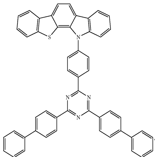
Compound E62
