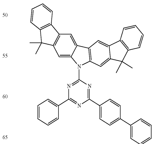
Compound E74
